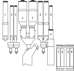
COFFEE BEANS X2 HOPPERS (valid configuration for version with traditional espresso brewer + version with variable chamber coffee brewer)
